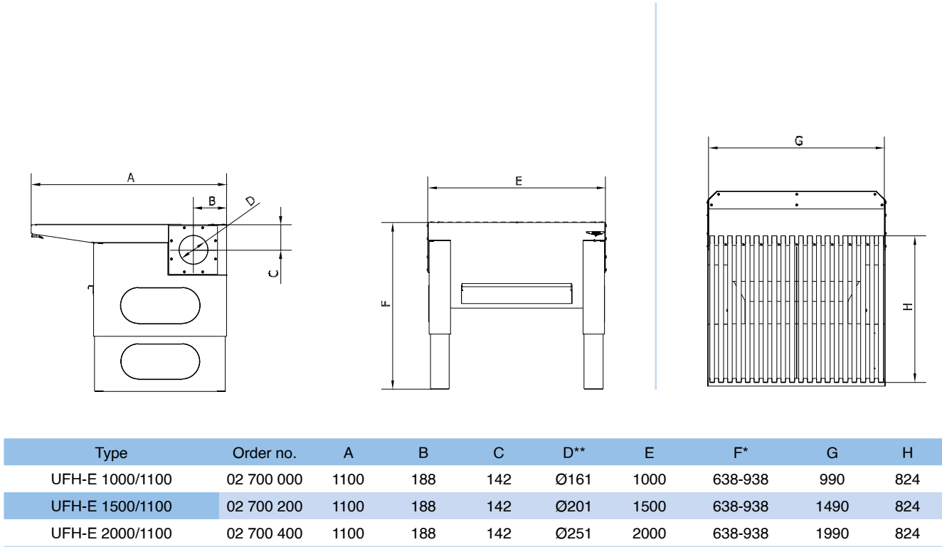
Extraction table type UFH-E:
