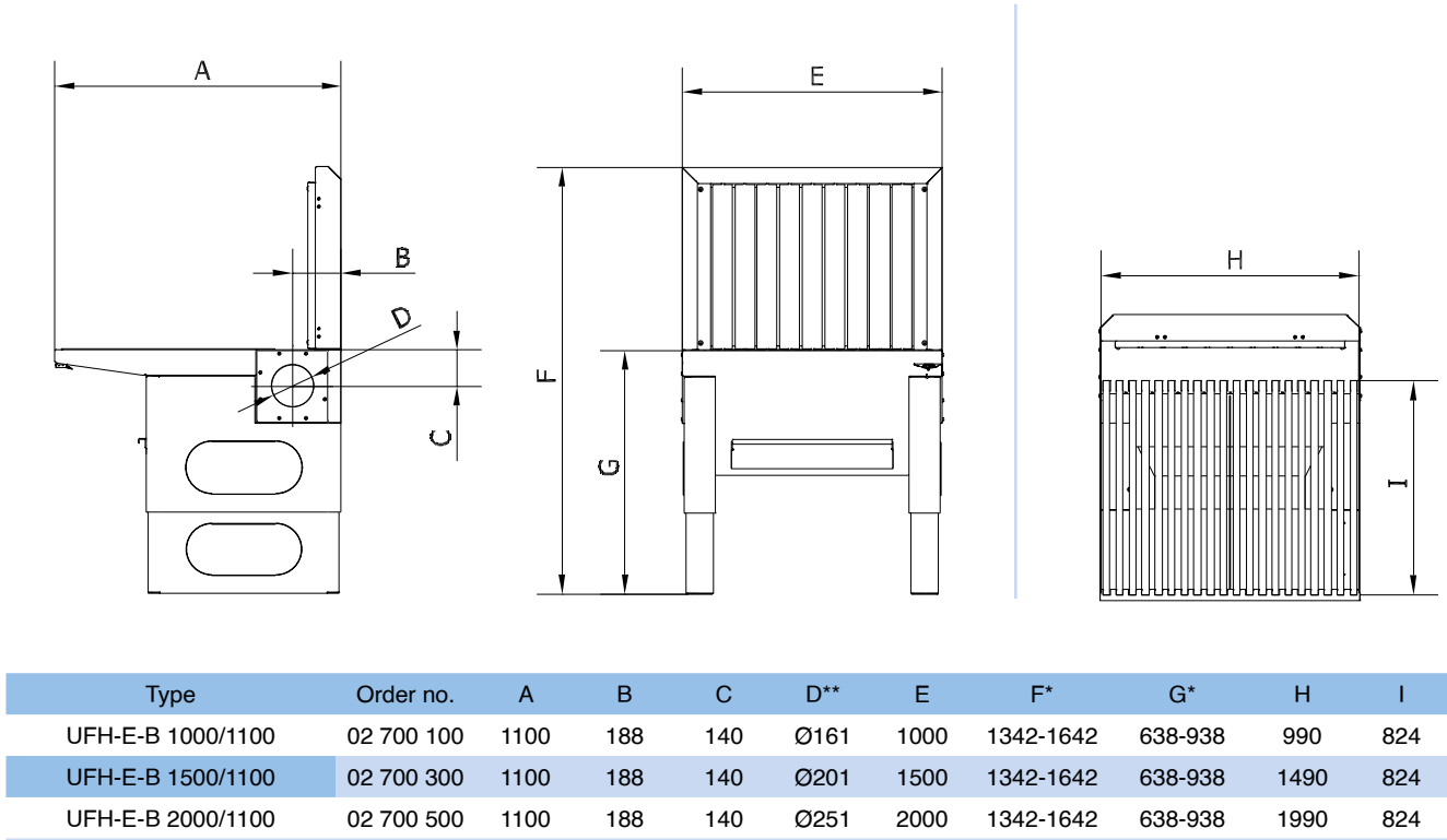
Extraction table type UFH-E-B - backwall with extraction:
